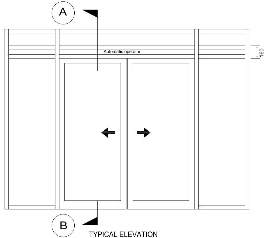
TYPICAL ELEVATION
